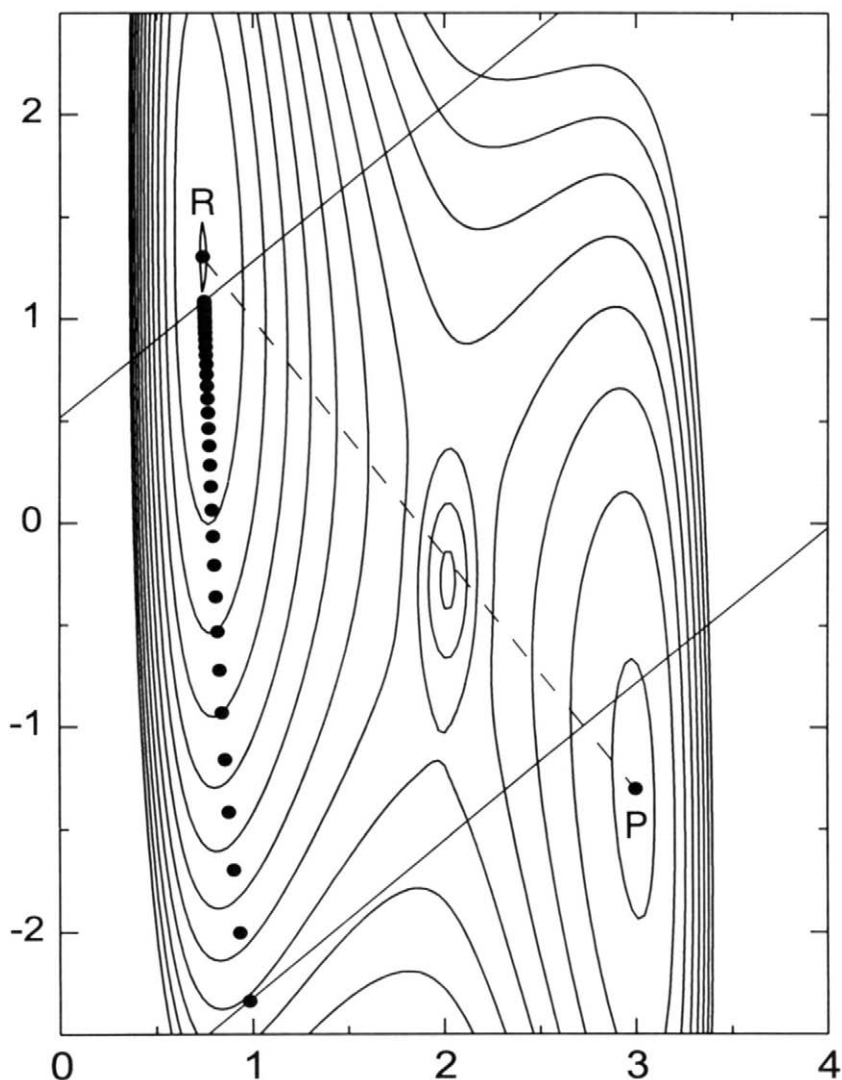
Figure 1 The 'drag' method. A drag coordinate is defined by interpolating from R to P with a straight line (dashed line). Starting from R , the drag coordinate is increased stepwise and held fixed while relaxing all other degrees of freedom in the system. In a two-dimensional system, the relaxation is along a line perpendicular to the P – R vector. The solid lines show the first and last relaxation line in the drag calculation. The final location of the system after relaxation is shown with filled circles. As the drag coordinate is increased, the system climbs up the potential surface close to the slowest ascent path, reaching a potential larger than the saddle point, and then, eventually, slipping over to the product well. In this simple test case, the drag method cannot locate the saddle point.
