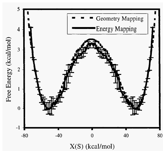
Figure 4. Comparison of computed potentials of mean force from the energy mapping (solid curve) and geometrical mapping (dash curve). The N-N distance was fixed at 2.7Å in all simulations.
