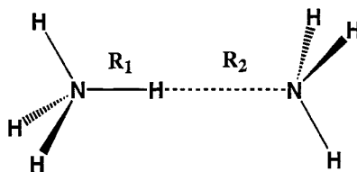
Figure 1 Schematic representation of the geometrical parameters for the [H_3N-H-NH_3]^+ ion. The reaction coordinate for the proton transfer is defined as X^R = 1/2[R_1 - R_2] .
