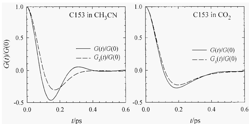
Figure 6. Solvation velocity TCFs (full line) and their single-molecule components (dashed line) for C153 in acetonitrile (left panel) and \text{CO}_2 (right panel) solvents. The system parameters are as in Fig. 2.
